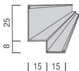
Tegular 15/90
